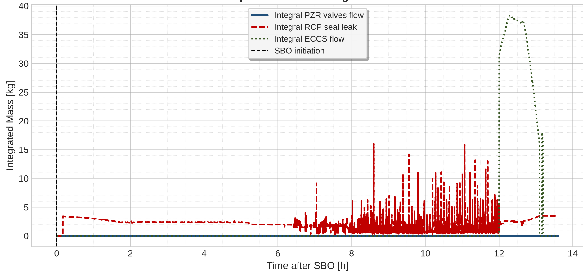
No SG Depressurization - Integral Mass Flows
